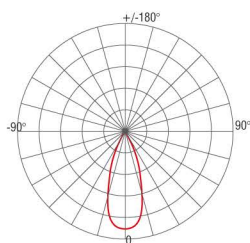
PHOTOMETRIC DATA
