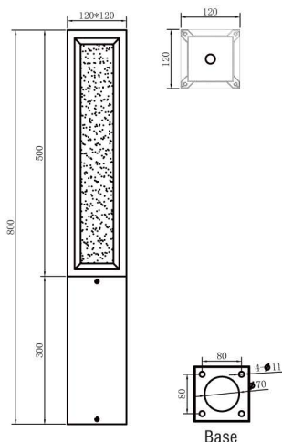
DIMENSION (Unit mm.)
