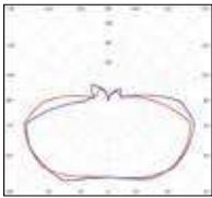
E27 (2450 lm) Real light output / frosted - 1633 lm
