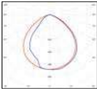
Model 1 LED 30W Real light output - 2716 lm CRI > 80
