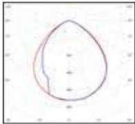
Models 2 to 4 LED 30W Real light output - 2691 lm CRI > 80
